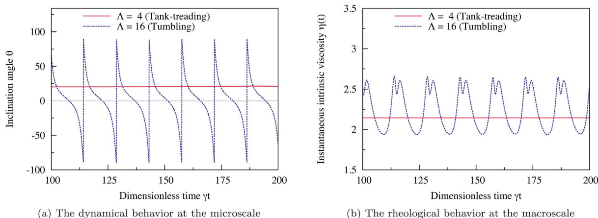
Fig. 1 (a) Evolution in time (rescaled time \gamma\tau ) of the inclination angle \theta (in degrees) of two vesicles: one in the TT state ( \Lambda = 4 ) and the other one in the TB state ( \Lambda = 16 ). The tank-treading vesicle assumes a steady inclination angle while the tumbling vesicle assumes a periodic angle. (b) The corresponding evolution in time of the instantaneous intrinsic viscosity \eta(t) in the TT state ( \Lambda = 4 ) and in the TB state ( \Lambda = 16 ). The vesicle in the TT regime performs steady motion and so does its viscosity. For the TB vesicle, the viscosity evolves in a periodic manner in time. The two figures recover qualitatively the same behavior as reported in ref. 7 computed with 2D boundary integral method simulations, in the limit of an unbounded suspending fluid ( \chi = 0 ). Here, the confinement is set to \chi = 0.2 . Other parameters are: Re = 0.5 , Ca = 10 , \Delta = 0.8 .
