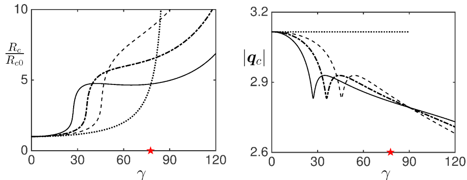
Figure 2: Critical Rayleigh number R_c , normalized to the value R_{c0} at \gamma = 0 (left panel) and critical wave number |\mathbf{q}_c| (right panel) as function of the inclination angle \gamma for Pr = 1.07 for different roll orientations \psi . Line styles for the different roll orientations are: \cdots for \psi = 90^\circ (longitudinal rolls, R_c^l(\gamma) ), --- for \psi = 60^\circ , - \cdot - for \psi = 45^\circ and — for \psi = 0^\circ (transverse rolls, R_c^t(\gamma) ). The codimension 2 point with \gamma_{c2} = 77.746^\circ is marked by a star.
