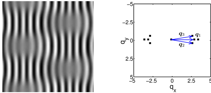
Figure 8: Transverse oscillatory rolls at Pr = 1.07 , \gamma = 84.9^\circ and \epsilon = 0.07 : temperature plot (left panel); wave vectors of the dominant Fourier modes (right panel). In this case, we use a square grid with q_y = q_c = 3.117 .
