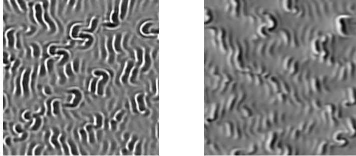
Figure 20: Chaotic switching rolls at \gamma = 100^\circ , \epsilon = 0.19 [experiments (left panel), simulations (right panel)].
