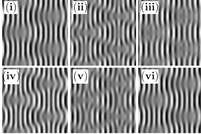
Figure 9: A time sequence of transverse oscillatory (TO) patterns shown over one time period for the case of heating from below. Consecutive panels are separated by 0.44t_\nu . System parameters are the same as figure 8 with Pr = 1.07 , \gamma = 84.9^\circ and \epsilon = 0.07 .
