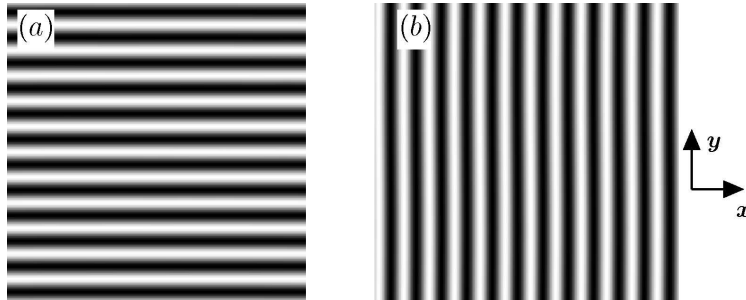
Figure 4: Temperature plots \langle \theta(\mathbf{x}) \rangle , for Pr = 1.07 from direct numerical simulations of the OBE (2.1): (a) buoyancy dominated longitudinal rolls (LR) oriented along the incline at Pr = 1.07 , \epsilon = 0.01 , \gamma = 10^\circ with \mathbf{q}_c = (0, 3.1163) (left panel); (b) shear dominated transverse rolls (TR) oriented perpendicular to the incline at \epsilon = 0.02 , \gamma = 85^\circ with \mathbf{q}_c = (2.82, 0) (right panel). See text for further details of the simulations. In the plane the figures are oriented along the x-axis of local coordinate system in figure 1 (reproduced at the right). All temperature plots in the rest of the paper are shown using the same convention.
