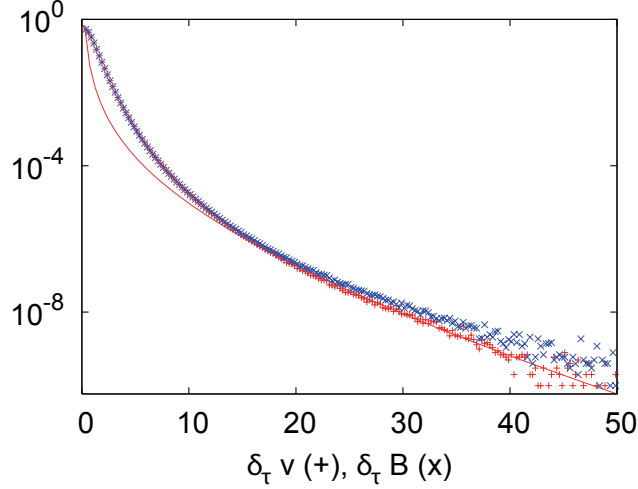
Figure 7. Comparison of PDFs of velocity(+) and magnetic field(x) increments for small \tau : magnetic field increment are broader. The continuous line corresponds to the multifractal approach.
