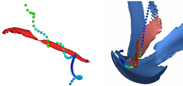
Figure 6. Trajectories with high acceleration in NS (left) and MHD (right, blue denotes current density and red vorticity).
