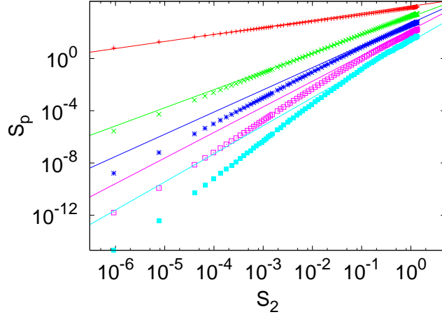
Figure 5. Lagrangian structure functions from Run4 of order 1,3,4,5,6 (top to bottom)
