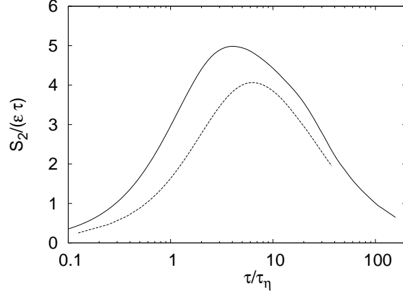
Figure 2. 2nd order structure function normalized to \epsilon\tau for Run1 (solid line) and Run4 (dashed line)
