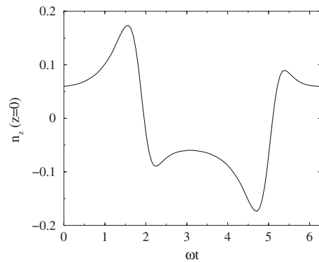
FIG. 4. Temporal evolution of the director amplitude n_z(0, t) over one period 0 < \omega t < 2\pi of the driving ac voltage.
