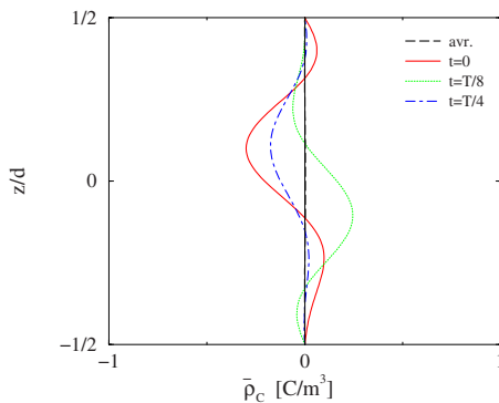
FIG. 7. (Color online) Profile of the amplitude of the Coulomb charge density \bar{\rho}_C = \bar{\rho}_{el} - \bar{\rho}_{fl} along z for different times.
