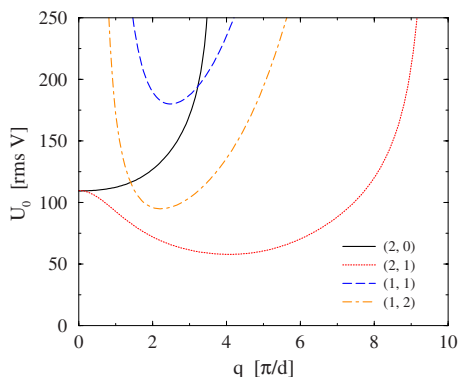
FIG. 9. (Color online) Neutral curves U_0(q) for the wave vector \mathbf{q}=(q,p) as a function of q at a fixed value of p for different magnitudes of the flexo coefficients (\xi_-, \xi_+) at \omega\tau_q=0.5 .
