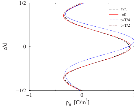
FIG. 6. (Color online) Profile of the amplitude \bar{\rho}_{fl}(z,t) of the flexo charge density along z for different times.
