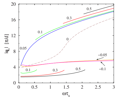
FIG. 2. (Color online) Modulus of the critical wave vector q_c as function of \omega\tau_q for different \sigma_a/\sigma_\perp .
