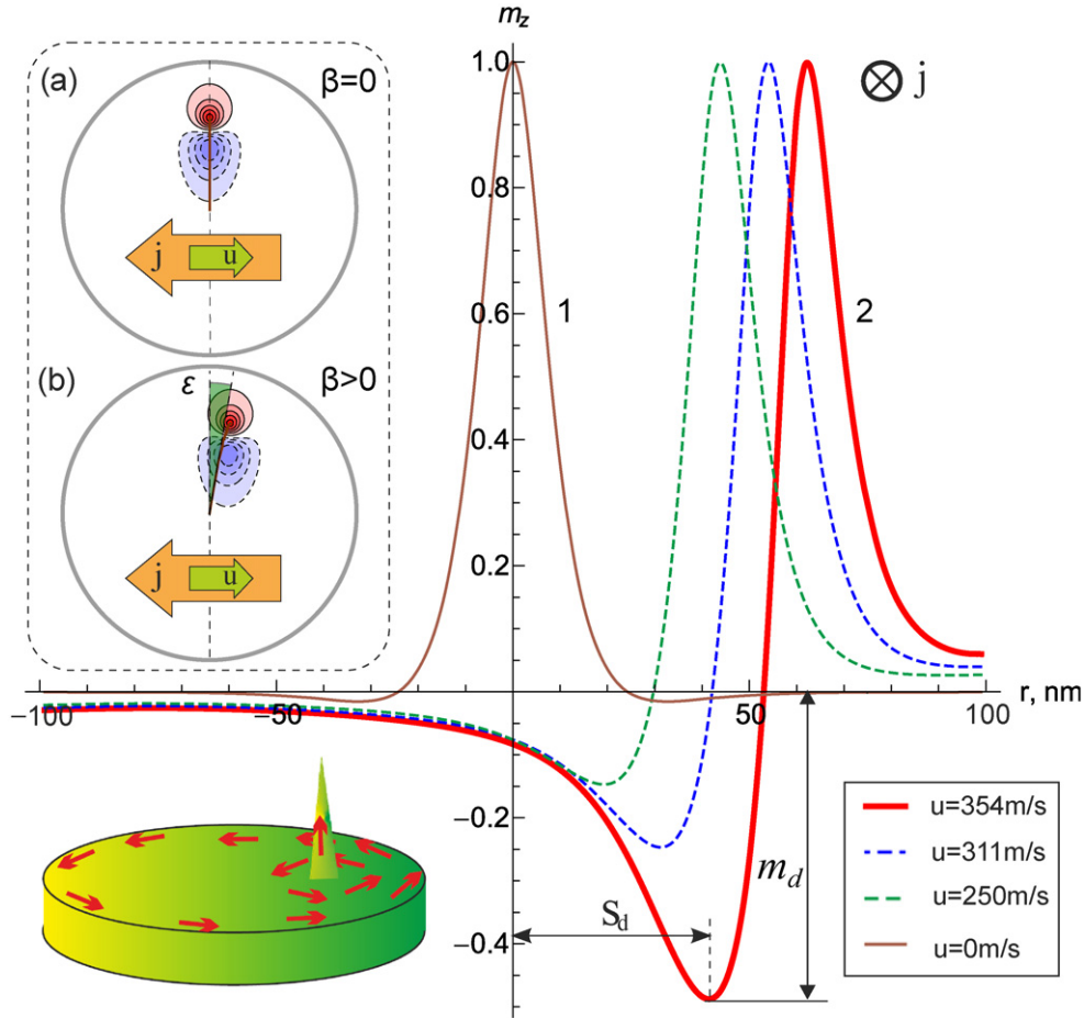
Figure 1. Profiles of the immobile equilibrium vortices for different values of the applied current. The profiles were taken along the diameter line perpendicular to the current direction (vertical dashed line on the insets) for case \beta = 0 . The insets demonstrate the 2D distribution of the out-of-plane magnetization for current close to critical one: \beta = 0 —inset (a) (the corresponding profile is shown with curve 2), and \beta = 0.1 —inset (b). Dashed isolines correspond to the case m_z < 0 and solid isolines—to m_z > 0 . Trajectory of the vortex core motion under adiabatically slow increasing of the current is shown as thick solid line in the insets. All presented data were obtained from the micromagnetic simulations of the permalloy nanodisc with radius L = 100 nm and thickness h = 20 nm.
