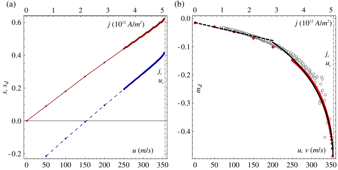
Figure 2. Parameters of the equilibrium vortex state depending on the applied current ( \beta = 0 ). (a) shows the vortex (solid line) and dip (dashed line) displacement from the disc centre depending on the velocity u . The displacements are measured in units of L . (b) shows dependence of the dip depth m_d on u : points represent the simulation data and the curve corresponds to equation (4). The open circles correspond to the dip amplitude of the vortex during its free gyromotion without current versus velocity of the vortex core v . The vertical dashed line denotes the critical current u_c when the vortex–antivortex pair is born.
