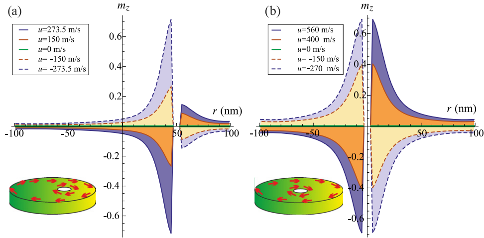
Figure 3. In-plane vortex profiles for different current values and vortex positions. Dashed and solid lines correspond to the opposite current directions. (a) shows profiles of the initially in-plane vortex pinned by the hole displaced by the value L/2 from the disc centre. (b) shows the similar profiles for the centred vortex. Simulations were performed for the permalloy disc with L = 100 nm and h = 10 nm for the case \beta = 0 .
