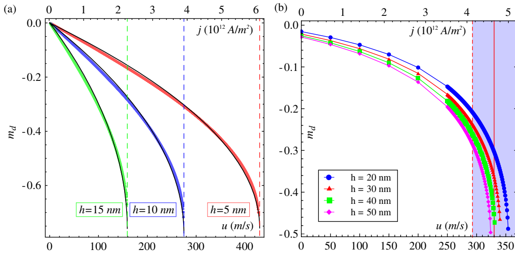
Figure 4. Dependences of the dip depth on the applied current for different thicknesses. (a) In-plane vortex is pinned on the hole with s = 0.5 , (b) free out-of-plane vortex. Solid black lines demonstrate the dependence (7). The critical velocity u_c = 330 \pm 37 \text{ m s}^{-1} which was determined in [35] is shown in the (b) as a vertical strip. The simulations are performed for samples with radius L = 100 \text{ nm} for case \beta = 0 .
